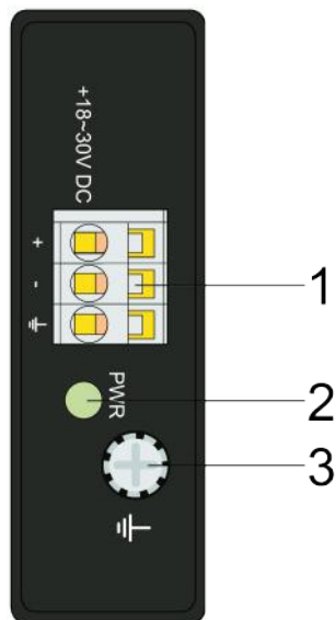
Figure 2: Top View of the Industrial ECO Switch
